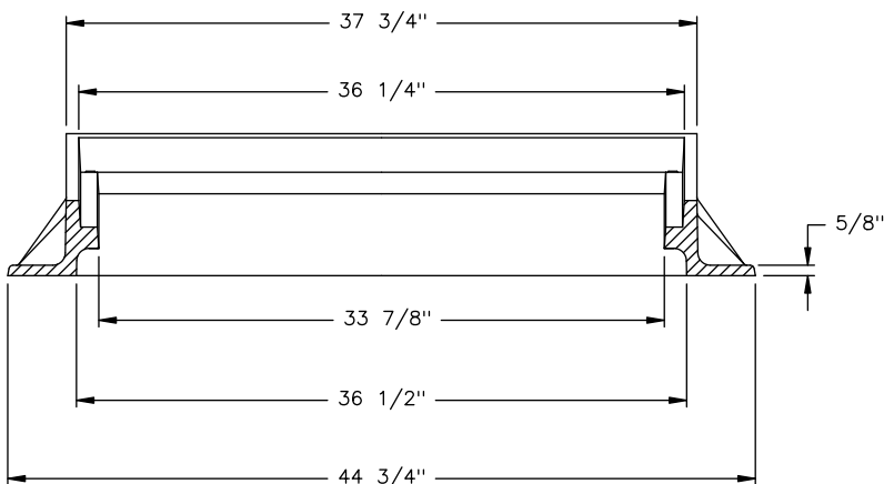
FRAME SECTION
