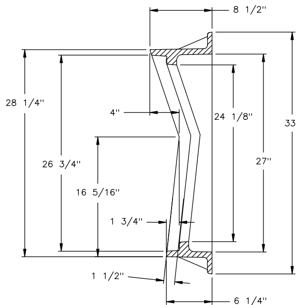
FRAME SECTION
